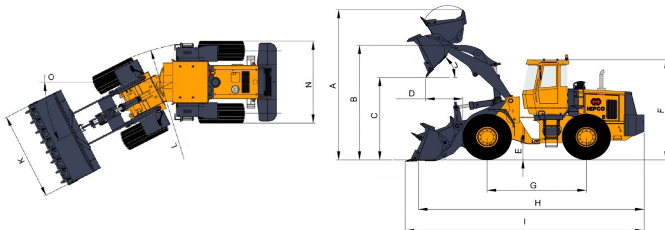
Dimension (mm)
